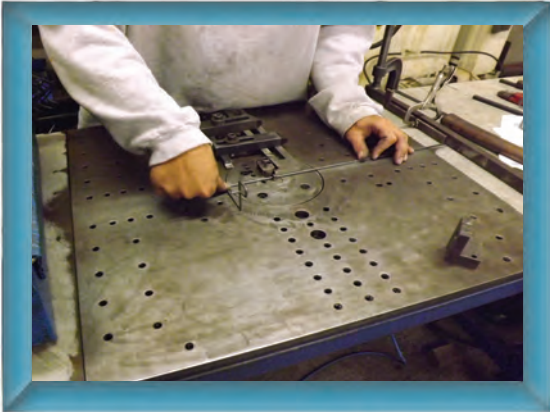
The Table Benders are capable of bending and forming wire .062" to 1".
